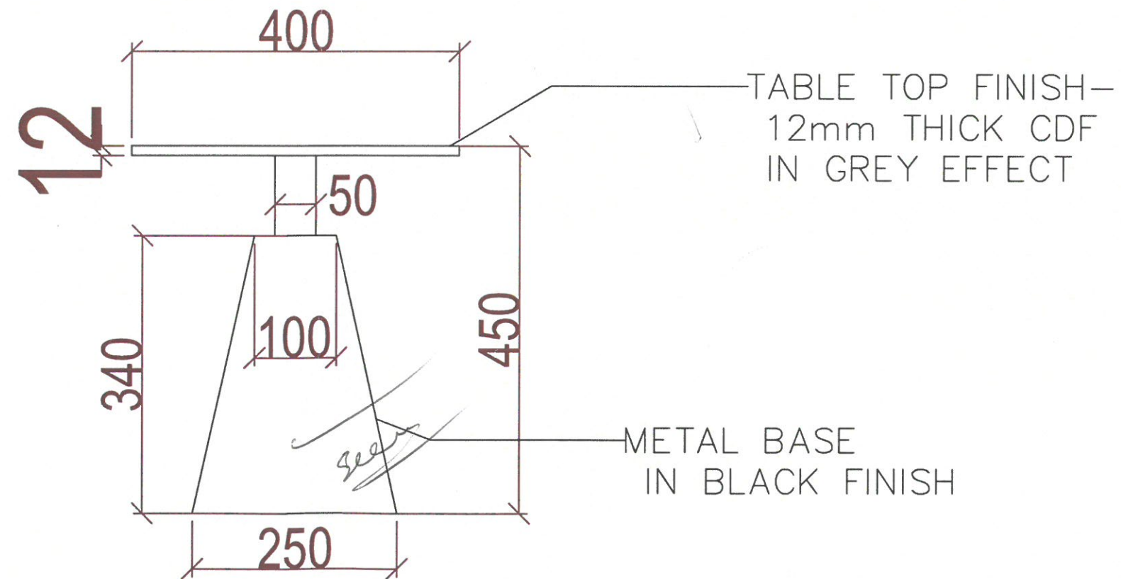
FRONT VIEW -SIDE TABLE
